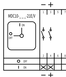
MDC10-040-1000-21 E/V IEC
