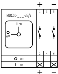
MDC10-040-1000-2 E/V IEC
