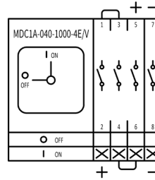
MDC1A 040-1000-4 E/V IEC UL
