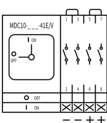
MDC10-040-1000-41 E/V IEC MDC40-160-1000-4 E/V IEC
