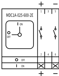
MDC1A 025-600-2 E IEC
